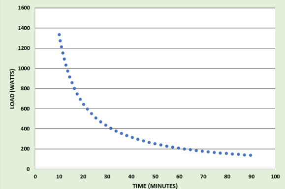
2U LFP BATTERY (Run Time vs Power) Room Temperature Conditions
